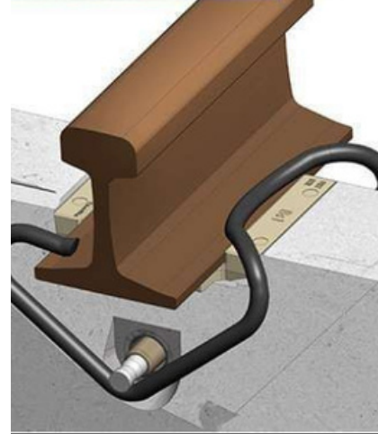
FIRST-CLIP ASSAMBLE
